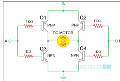
Figure 9. H Bridge to drive the DC motor [12]
