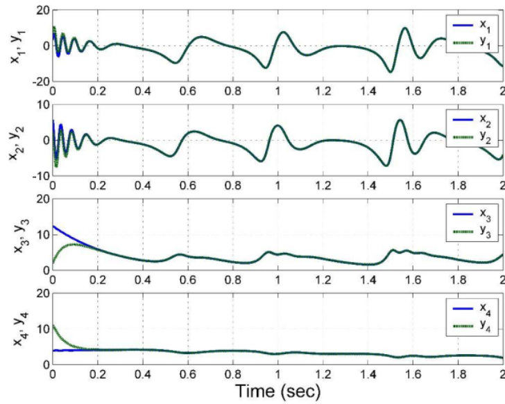
Figure 4. Complete synchronization of the hyperchaotic systems (14) and (15)
