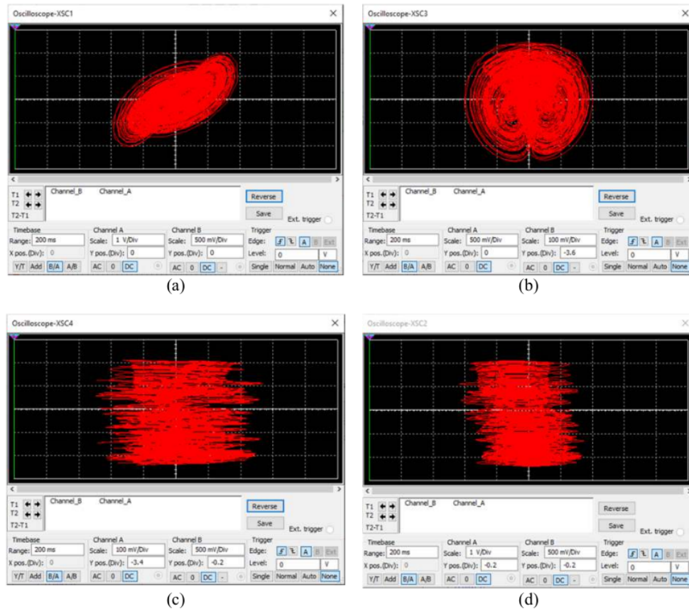
Figure 7. MultiSIM chaotic attractors of the new hyperchaotic two-scroll system (a) x_1 - x_2 plane, (b) x_2 - x_3 plane, (c) x_3 - x_4 plane and (d) x_1 - x_4 plane.
