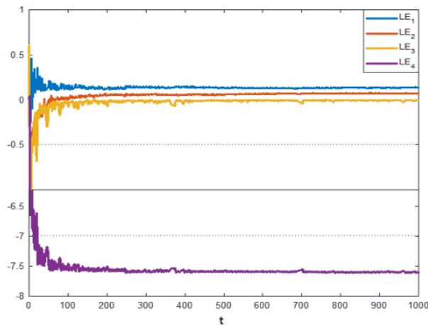
Figure 3 Lyapunov exponents of the new system (1) for the parameters values (2) and the initial conditions (3)
