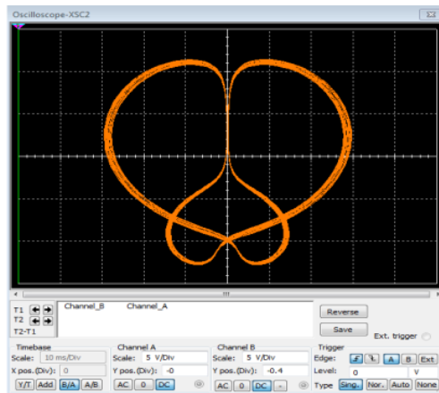
Figure 12 Multisim result of the x-z quasi-periodic orbit
