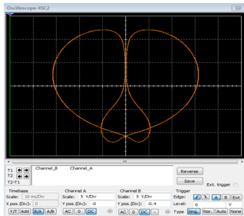
Figure 11 Multisim result of the x-z periodic orbit
