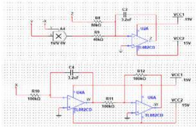
Figure 11. Circuit design for the new hyperchaotic system (1)
