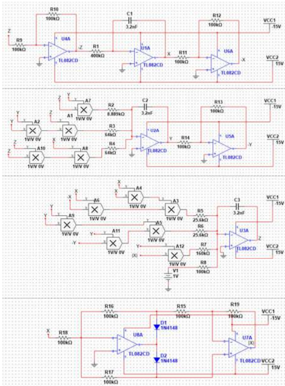
Figure 11. Circuit design for the new chaotic system (1)
