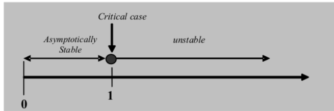
Figure 3 Stability at E_1(0,0,0)
