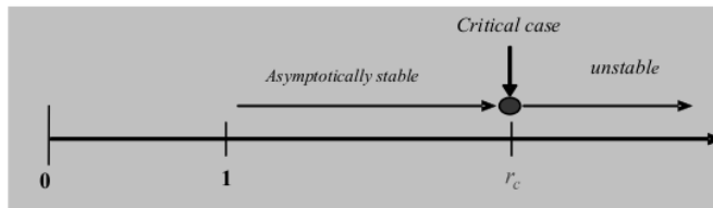
Figure 4 Stability at E_2(\sqrt{\beta(r-1)}, \sqrt{\beta(r-1)}, r-1)
