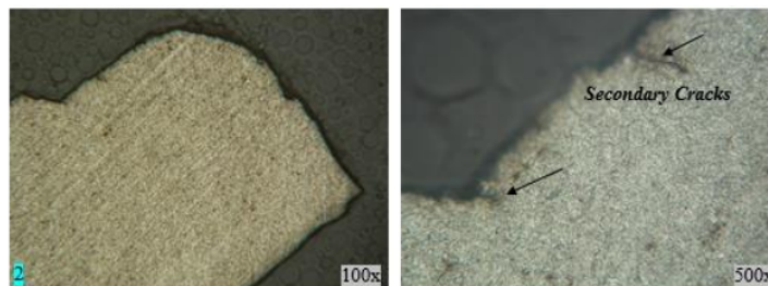
Figure 8. No.2 100x and 500x magnification.
