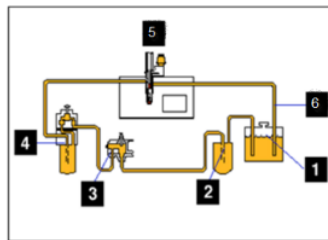
Figure 3. Fuel line diesel engine.
