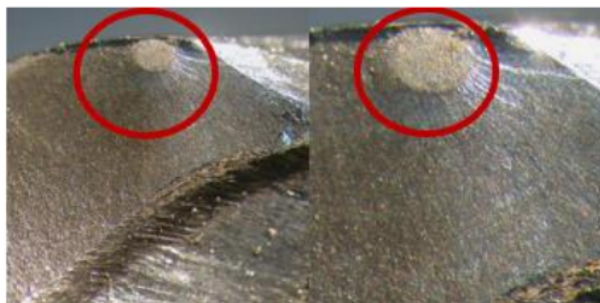
Figure 7. Benchmark injector spring fault.
