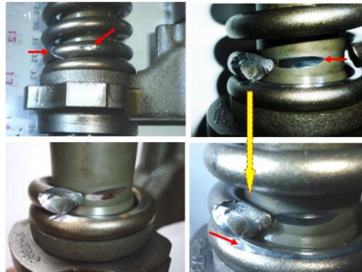
Figure 5. Photo macro on the injector fracture surface.
