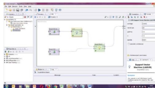
Figure 5. Algorithm modelling.
