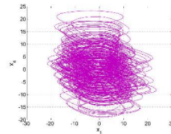
Figure 4. 2-D plot of the new hyperchaotic system (1) in the (x_1, x_4) plane for X_0 = (0.1, 0.1, 0.1, 0.1) and (a, b, c, d) = (30, 15, 3, 2)
