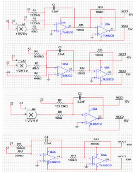
Figure 8: Circuit design of the new hyperchaotic system (1)
