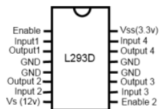
Figure 7. L293D pin configuration
