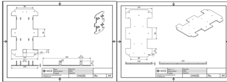
Figure 2. Frame
