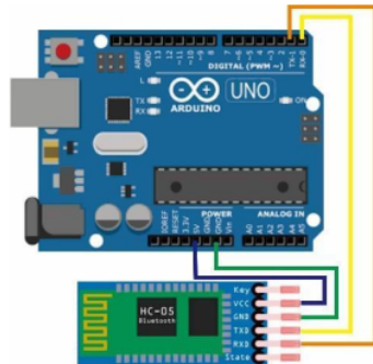
Figure 14. Bluetooth wiring on Arduino UNO
