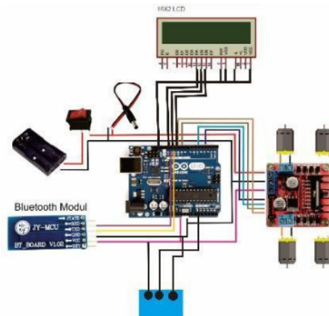
Figure 1. Scheme of metal detection robot
